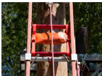
Buck Ladder Lock System (Bottom & Top) 355BT
